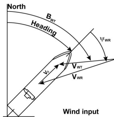
Figure 4 Sign convention for wind directions
