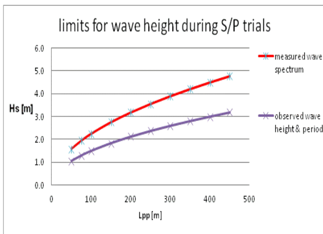
Figure 1; Limits for allowable wave height
